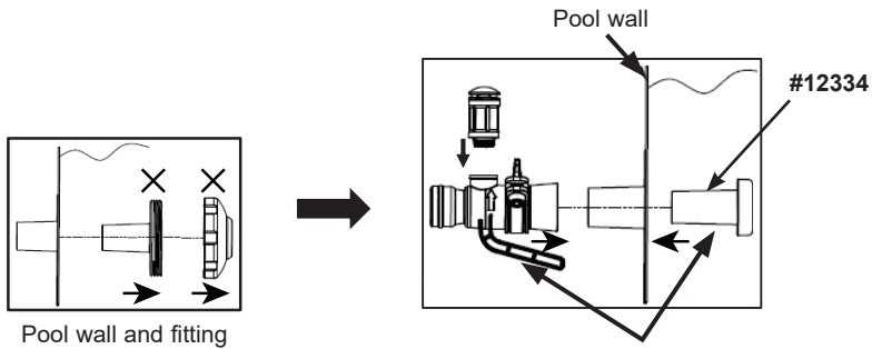
Intex Hydro Aeration inlet fitting
