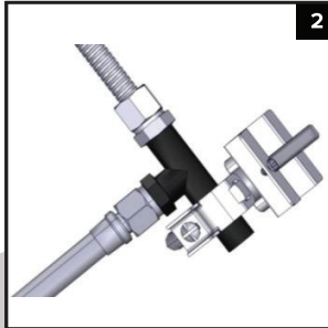
Turn the wheel clockwise to detach the regulator assembly from the cylinder valve.
